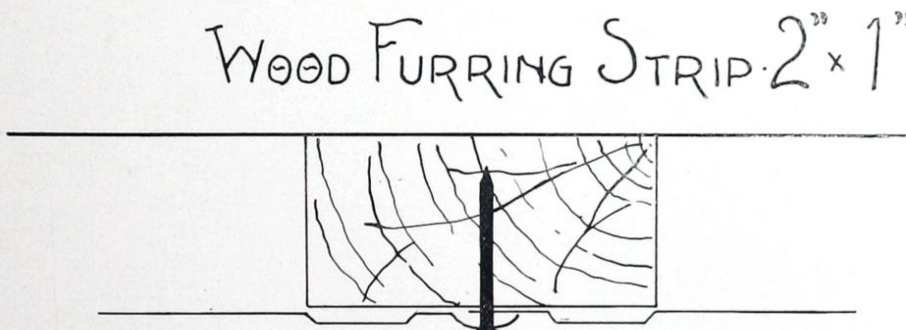
Fig. 3408.—Section of Joint on Plate No. 424.
